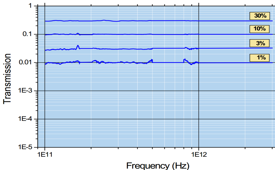
Attenuator Set Transmission
